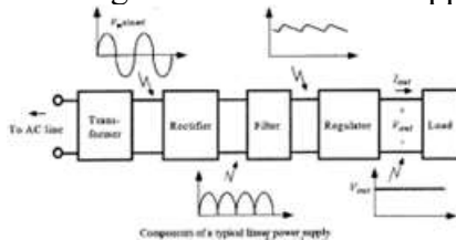
Fig:2. Block Diagram of Power Supply LCD DISPLAY
